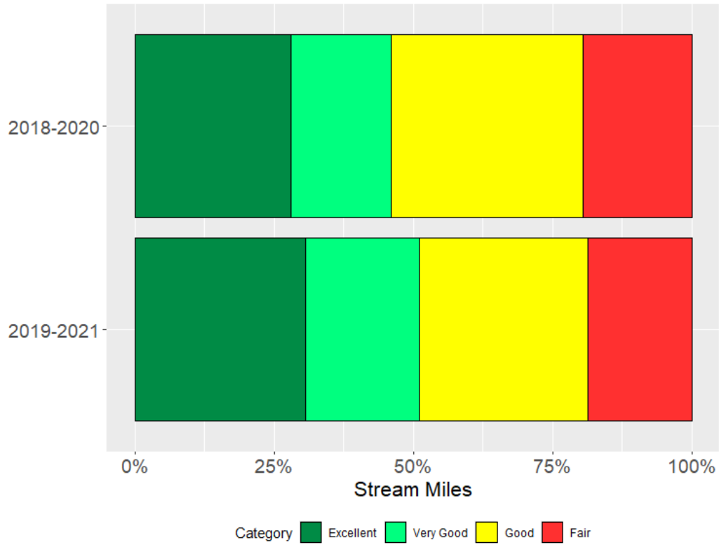
Figure 6. Estimates of the percentage of stream miles in each assessment category for macroinvertebrate communities from the past two probabilistic surveys.
