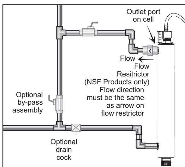
Figure 4 Flow Restrictor
