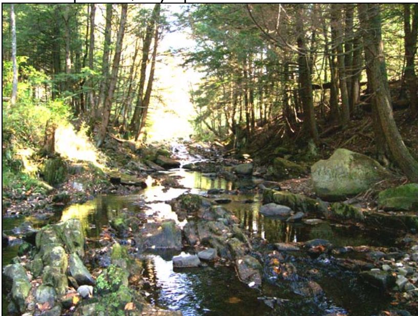
Centerville Brook segment R15.04-A is a bedrock gorge.
