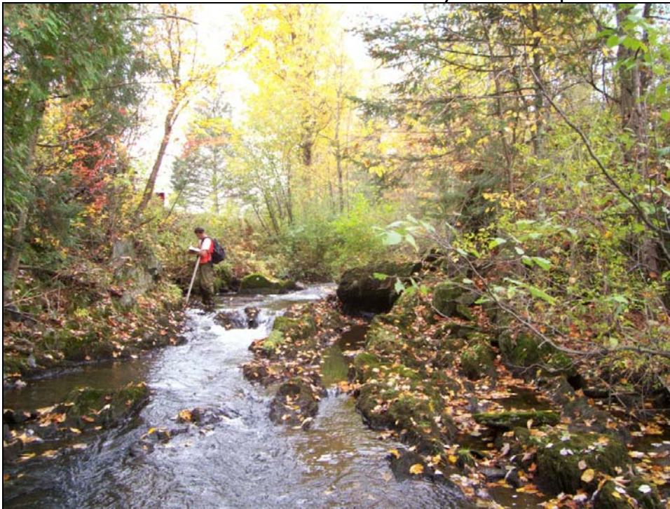
Centerville Brook segment R15.05-D is controlled by bedrock on the bed and banks.
