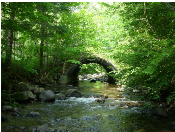
Figure 64. Turkey Hill Rd. stream crossing in reach T1.07 is undersized but is an excellent design for fish and other aquatic organism passage.
