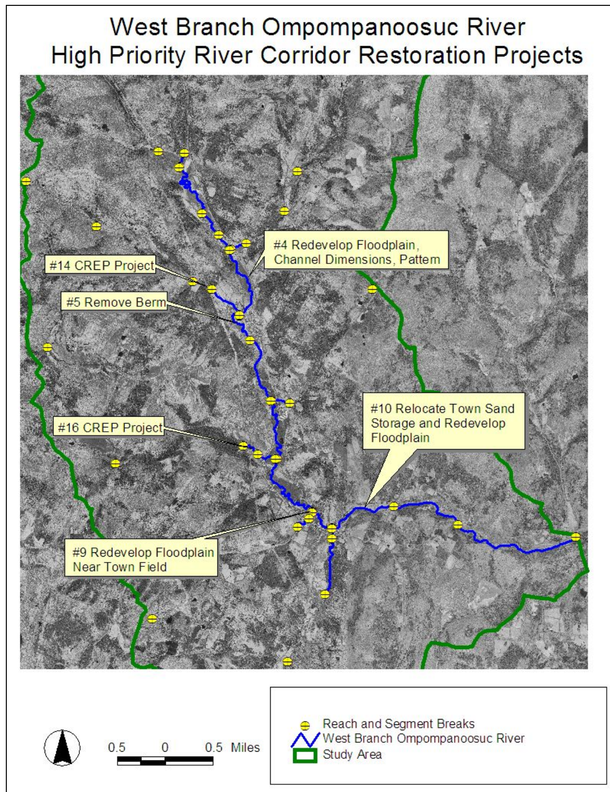
Figure 19: Project study area map of recommended projects.
