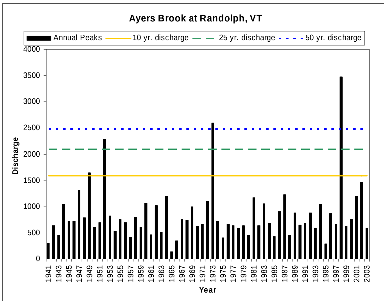
Figure 3: Flood frequency analysis for USGS 01142500 Ayers Brook at Randolph Vermont. Peak streamflow data from 1940 through 2003 were used in the analysis.
