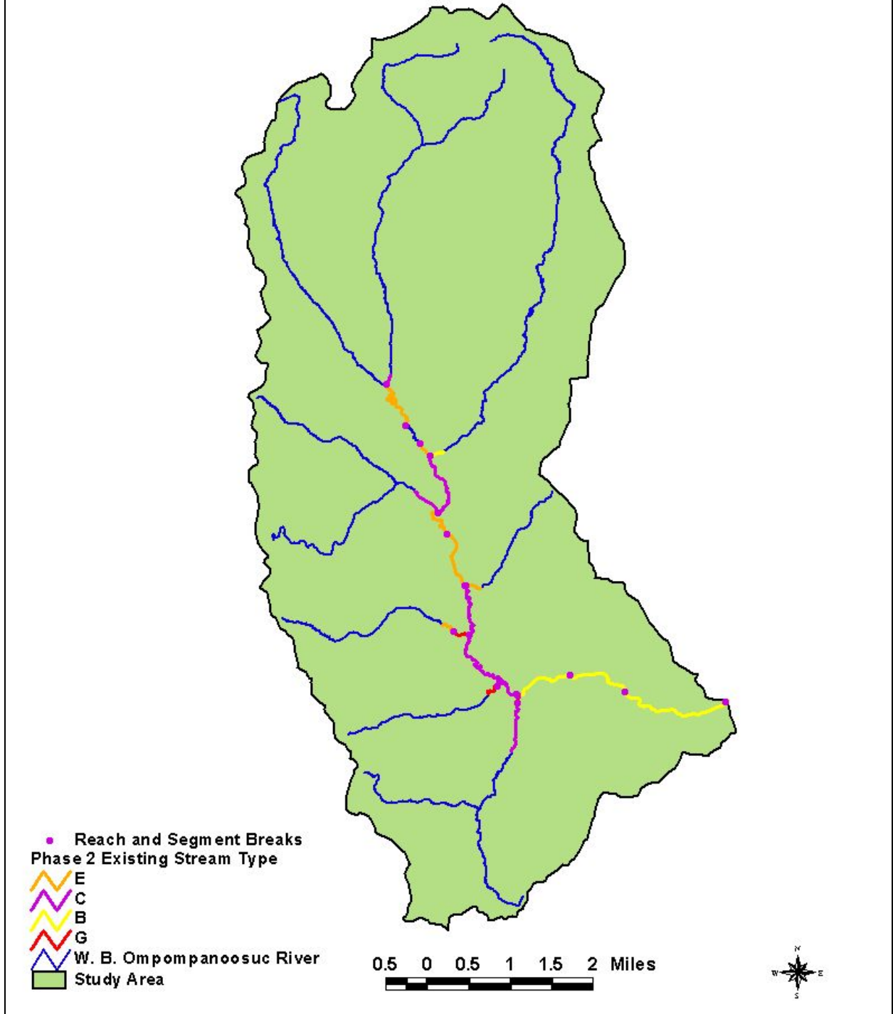
Figure 11. Phase 2 Existing Stream Types
