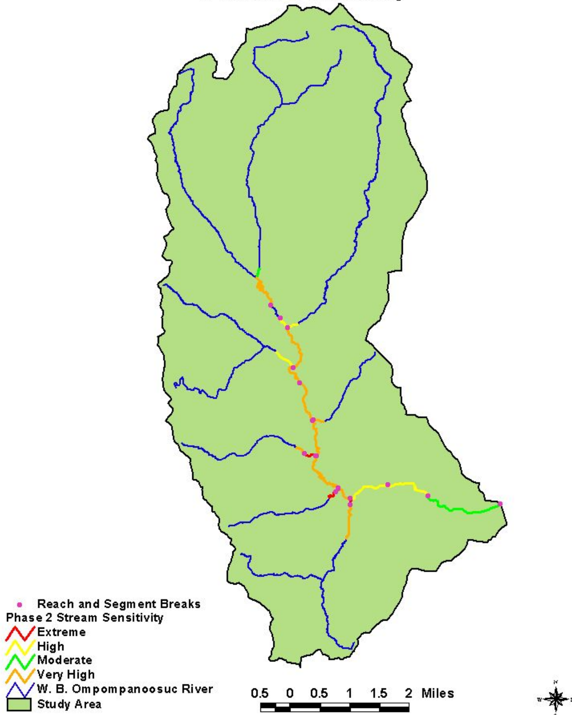
Figure 12: Phase 2 Stream Sensitivity Map
