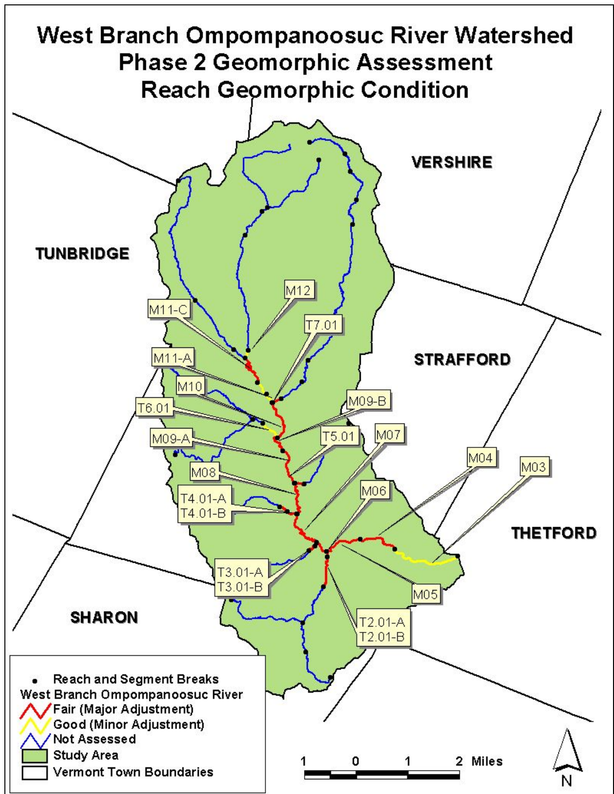
Figure 7: Phase 2 Geomorphic Condition of the West Branch Ompompanoosuc Watershed
