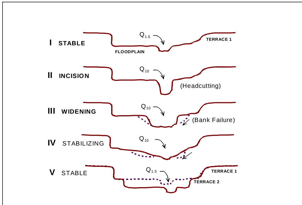
Figure 10: Typical Channel Evolution Model following incision.
