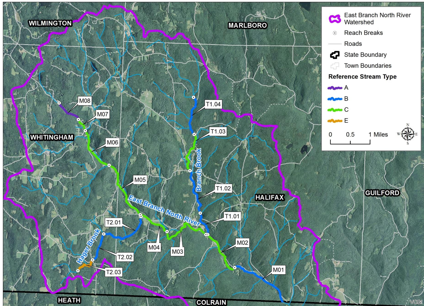
Figure 3.1: Reference stream types per Rosgen (1994) for the East Branch North River watershed.
