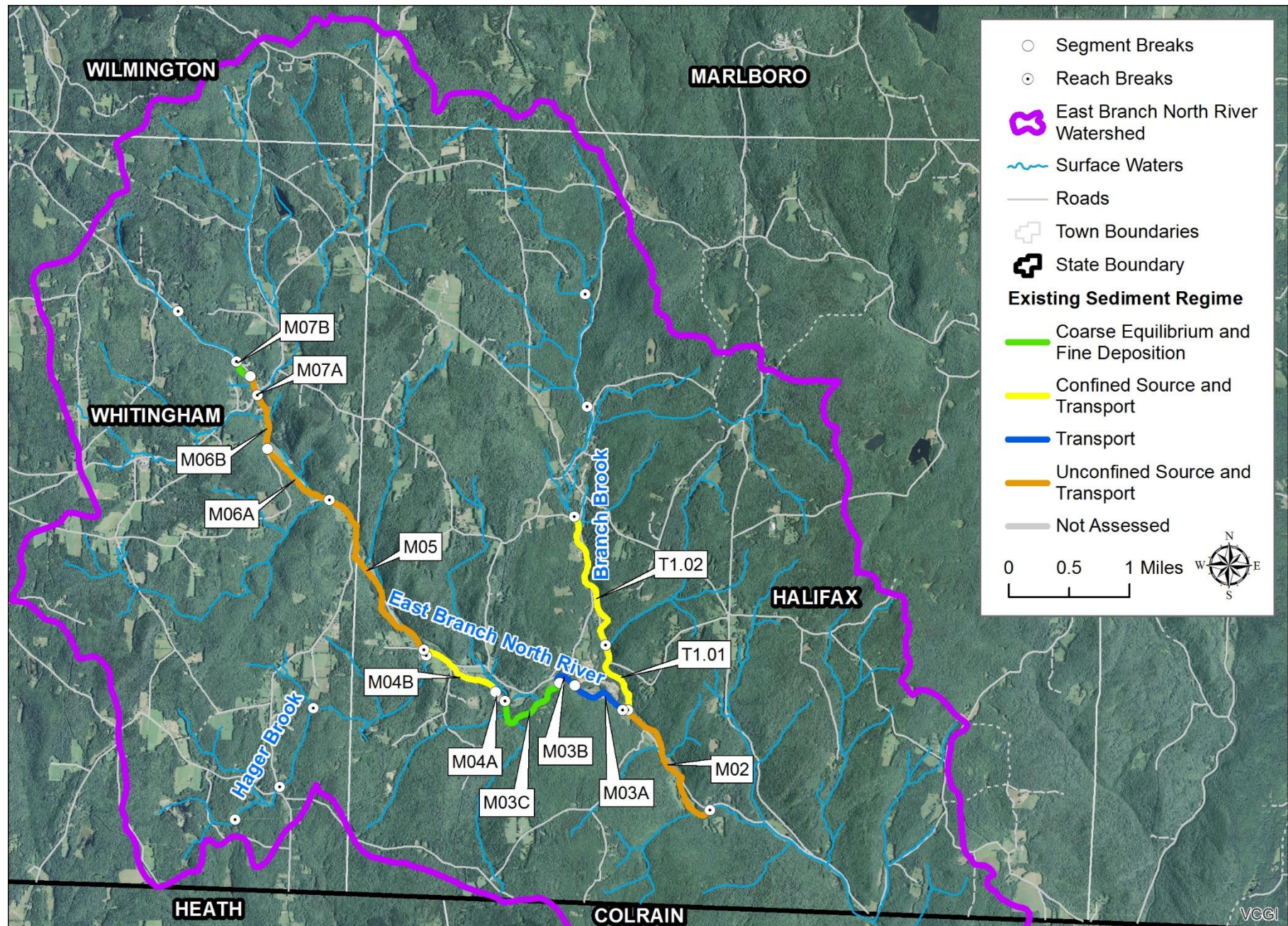
Figure 4.25: Existing Sediment Regime for the East Branch North River watershed.
