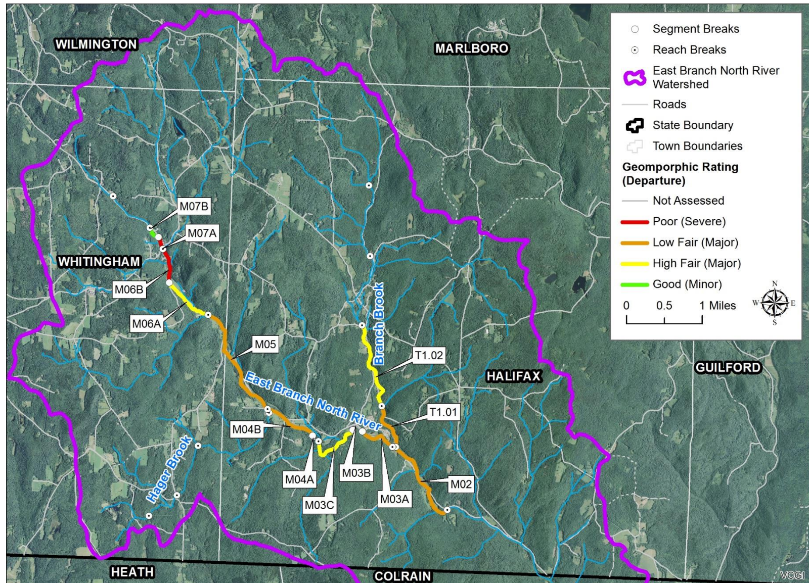
Figure 4.5: Rapid Geomorphic Assessment Ratings for the East Branch North River Watershed.
