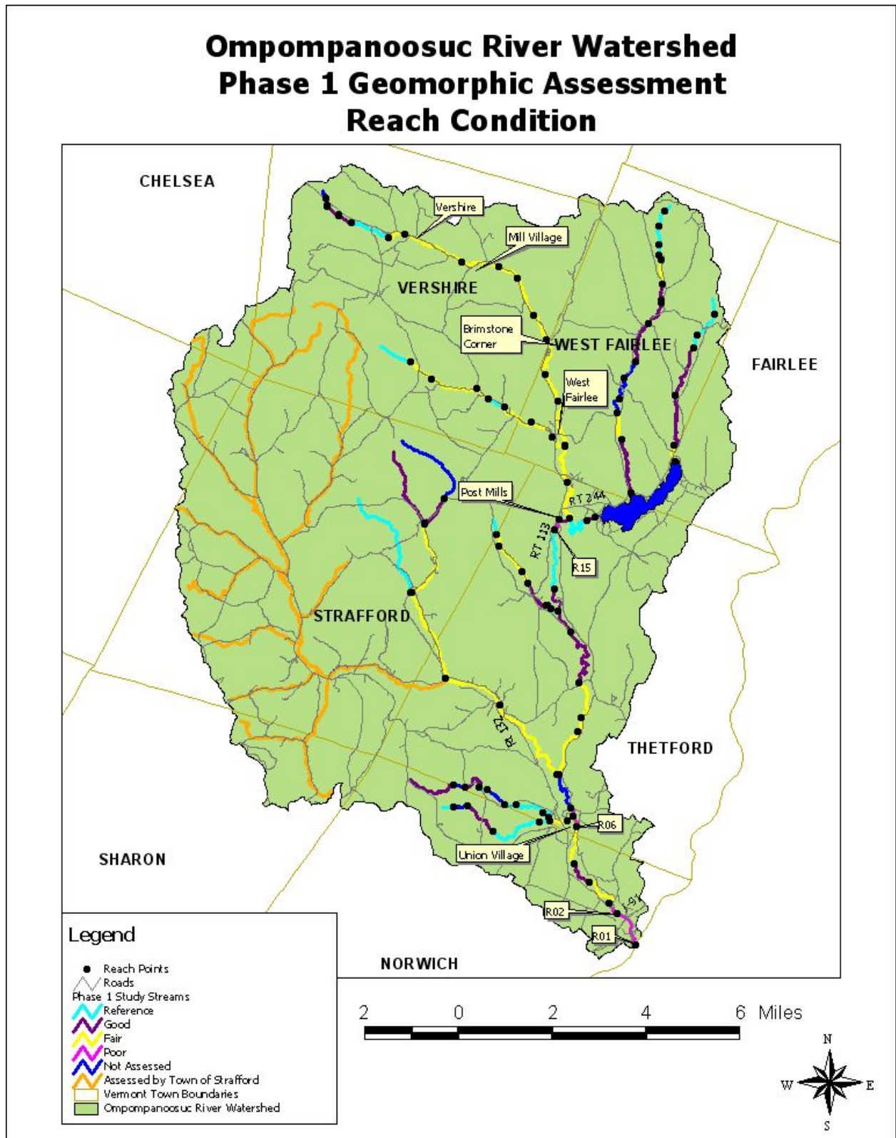
Figure 10: Reach Condition in the Ompompanoosuc River Watershed
