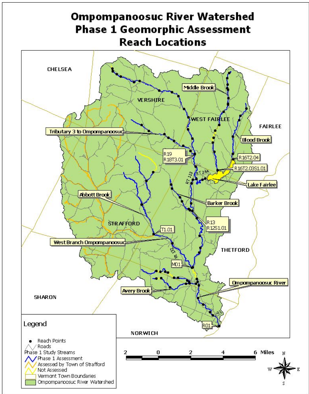
Figure 4. Ompompanoosuc River Watershed Reach Location Map for Stream Geomorphic Assessment
