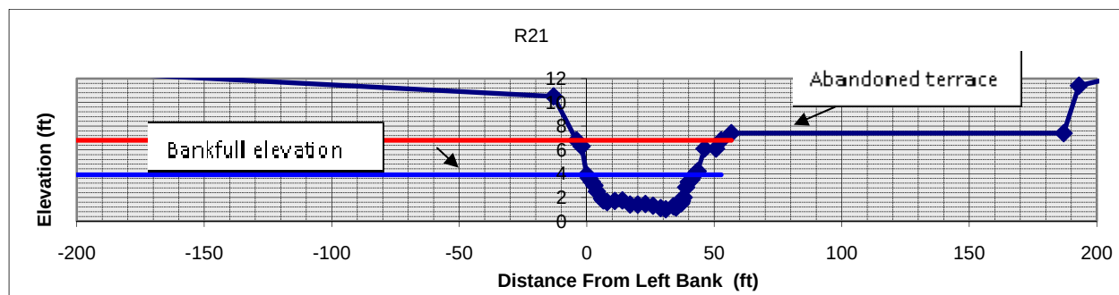
Figure 4.23 Channel cross section for segment R2I-A (graph is vertically exaggerated for illustration purposes)
