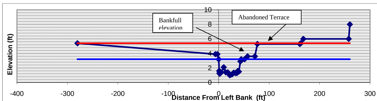
Figure 4.63 Graph of channel cross section for segment R18T3.01-A (The graph is vertically exaggerated for illustration purposes.)
