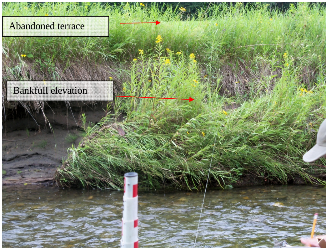
Figure 4.22 Cross section measurement in segment R21-A, showing incised channel.
