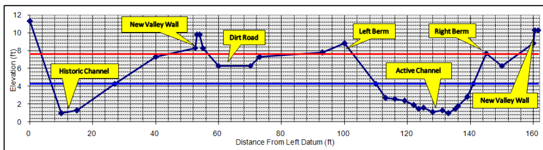
Figure 4.86 Cross-section of Willie Brook, showing historic channel and modified valley width
