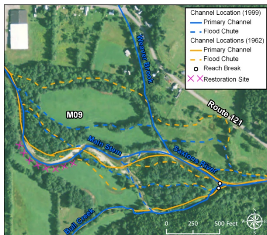
Figure 4.21 Channel migration and braiding in the last 50 years
