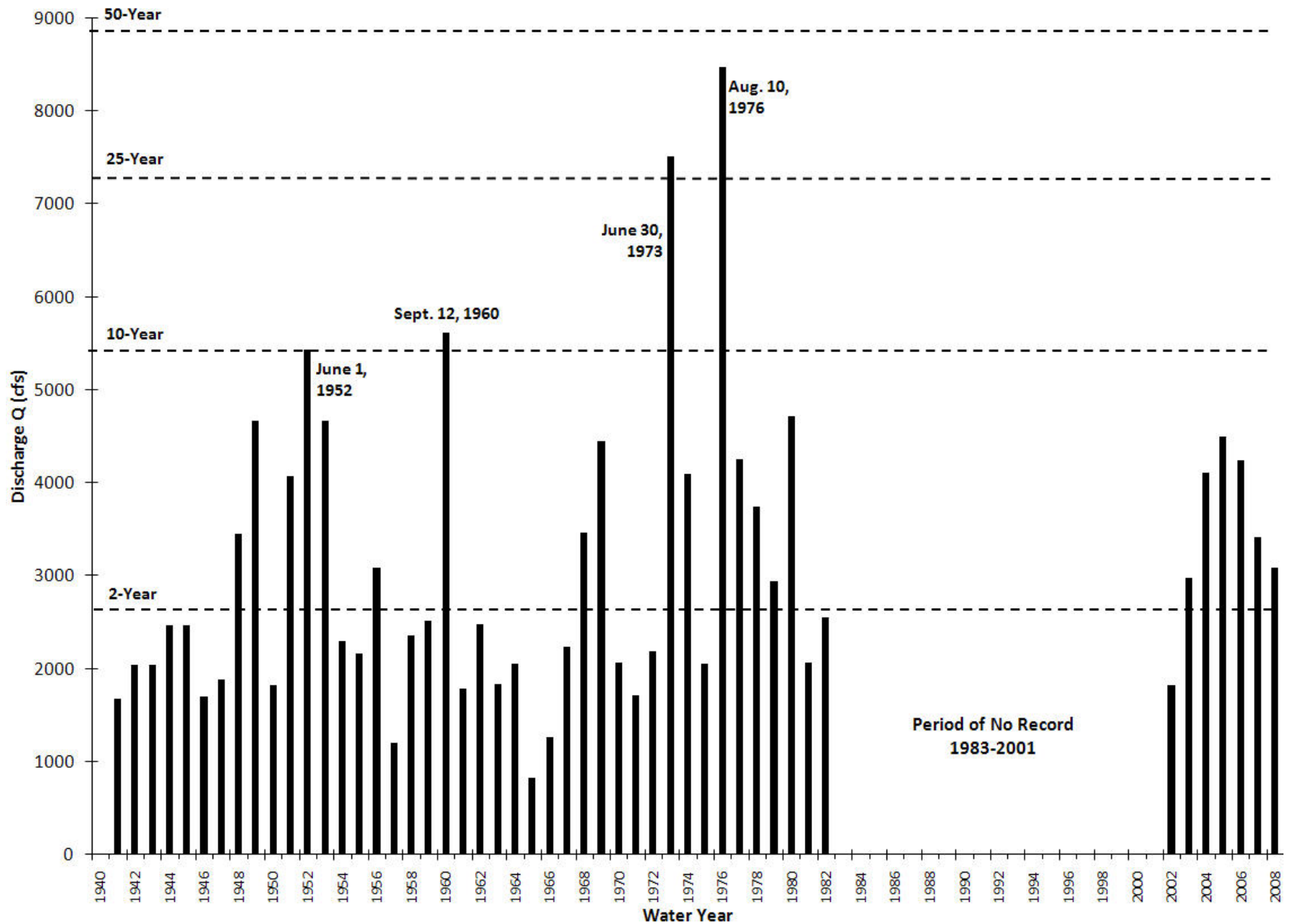
Figure 2.5 Annual peak discharges for USGS Gage # 01154000 on the Saxtons River in Windham County, Vermont; Recurrence intervals from Olson (2002)
