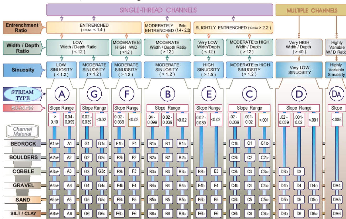
Figure 2.4 The Rosgen (1994) classification of streams based on channel morphology. Key parameters for classification include 1) the entrenchment ratio (floodprone width / bankfull channel width), 2) width to depth ratio (bankfull width / mean channel depth), and 3) channel sinuosity (channel length / straight-line valley length). Entrenched channels are typically dominated by sediment transport processes, whereas slightly entrenched channels (C and E types) have sediment transport and depositional processes.
