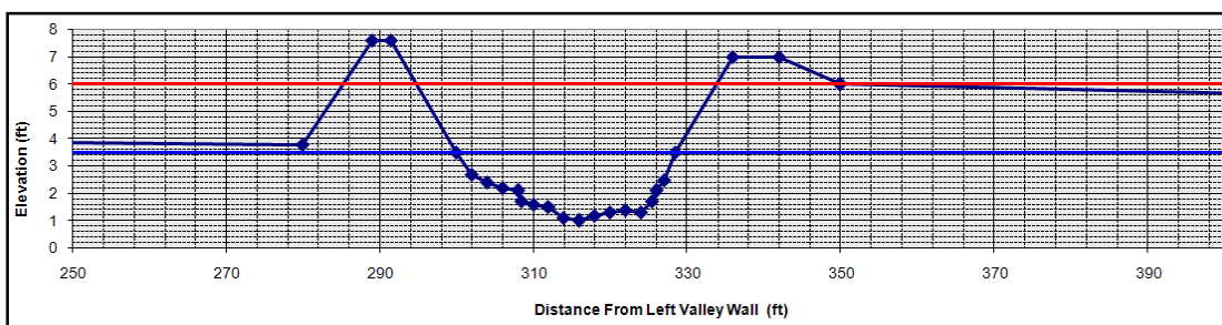
Figure 4.82 Cross-section of Willie Brook, showing berms along both channel banks
