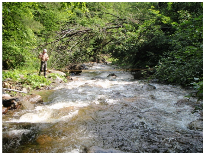
Figure 4.45 M20-A cross-section looking downstream
