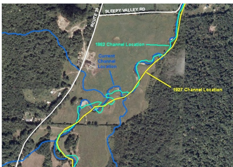
Figure 4.49 Historical channel straightening and redevelopment of meanders in T4.01-A, lower Bull Creek
