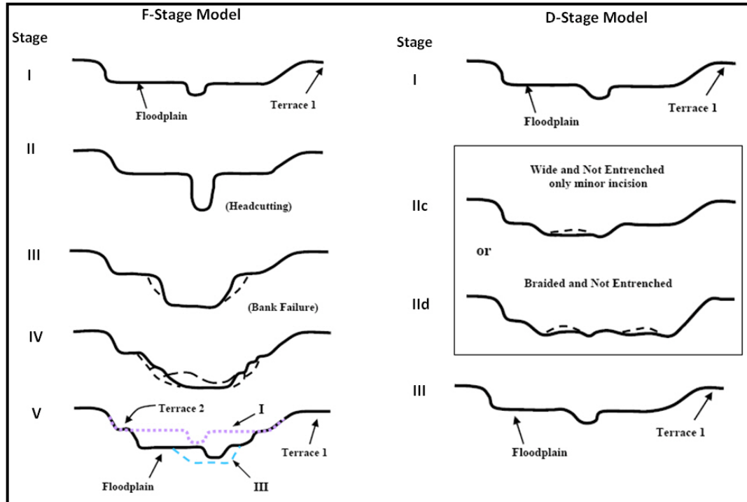
Figure 3.1 Typical channel evolution models for F-stage and D-stage (VTANR, 2009a)
