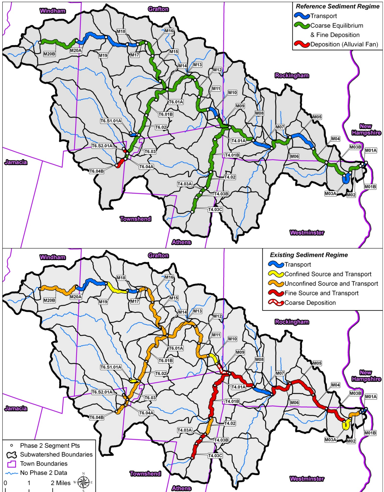
Figure 4.90 Reference and Existing Sediment Regime Maps for the Saxtons River
