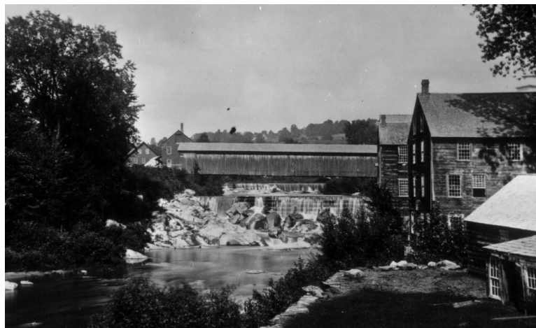
Figure 2.8 Upstream view of Westminster Street crossing and two crib dams (c. 1870 to 1949)
