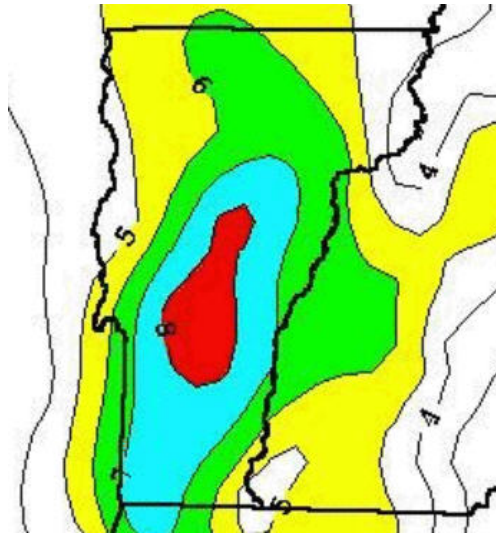
Figure 2.6 NWS Northeast River Forecast Center's predicted rainfall distribution during the 1927 flood in inches (NOAA, 2007)
