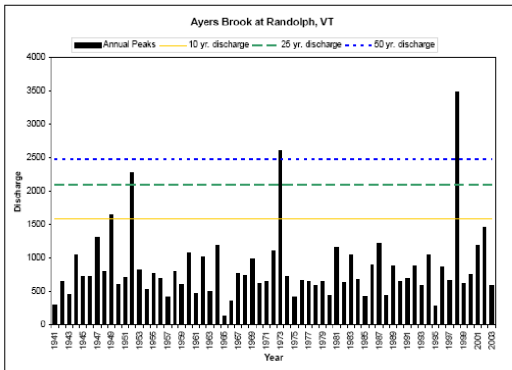
Figure 6. Annual and flood-level peak streamflows at the USGS continuous record stream gage on Ayers Brook. (Water years run from Oct. 1 to Sept. 30.)
