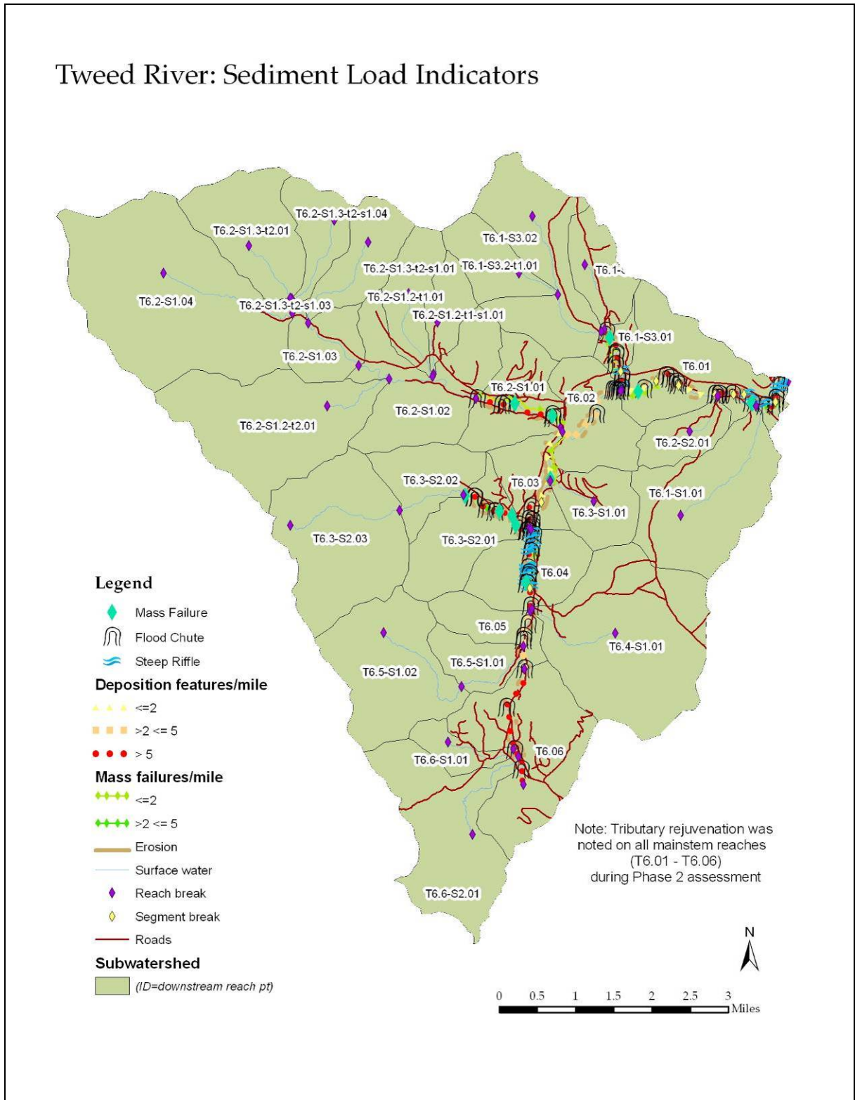
Figure 9. Watershed-scale sediment load indicators map for the Tweed River watershed.
