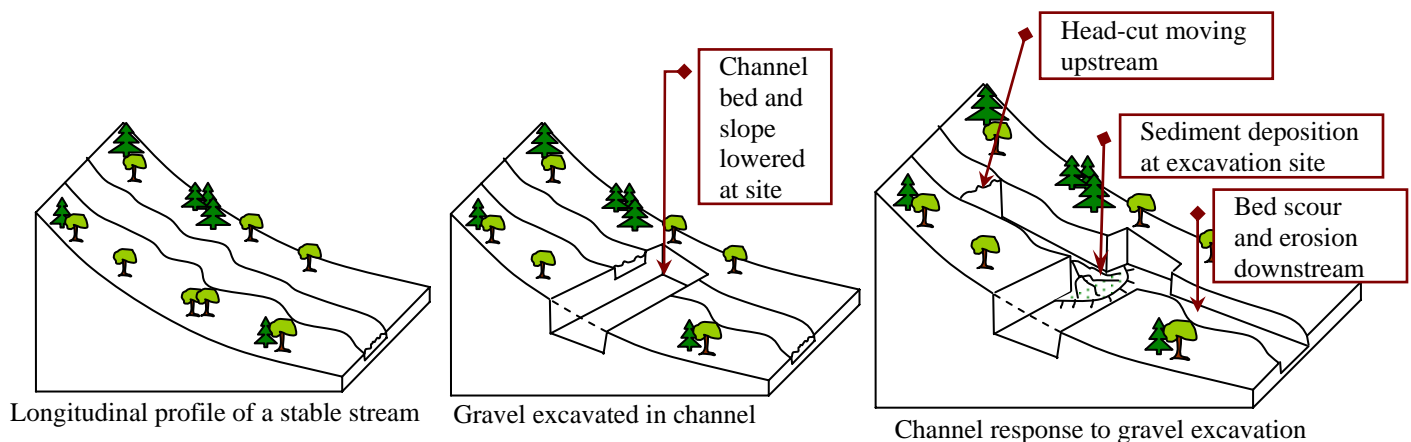
Figure 1: View of potential channel response due to gravel excavation. (Reproduced with permission Field, 2002)
