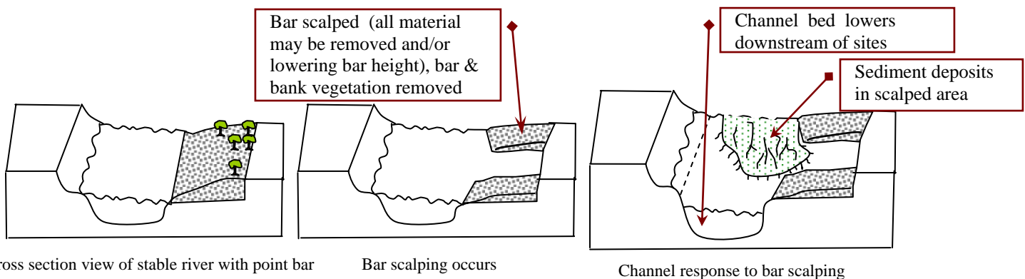
Figure 2: View of potential channel response due to bar scalping. (Reproduced with permission Field, 2002)
