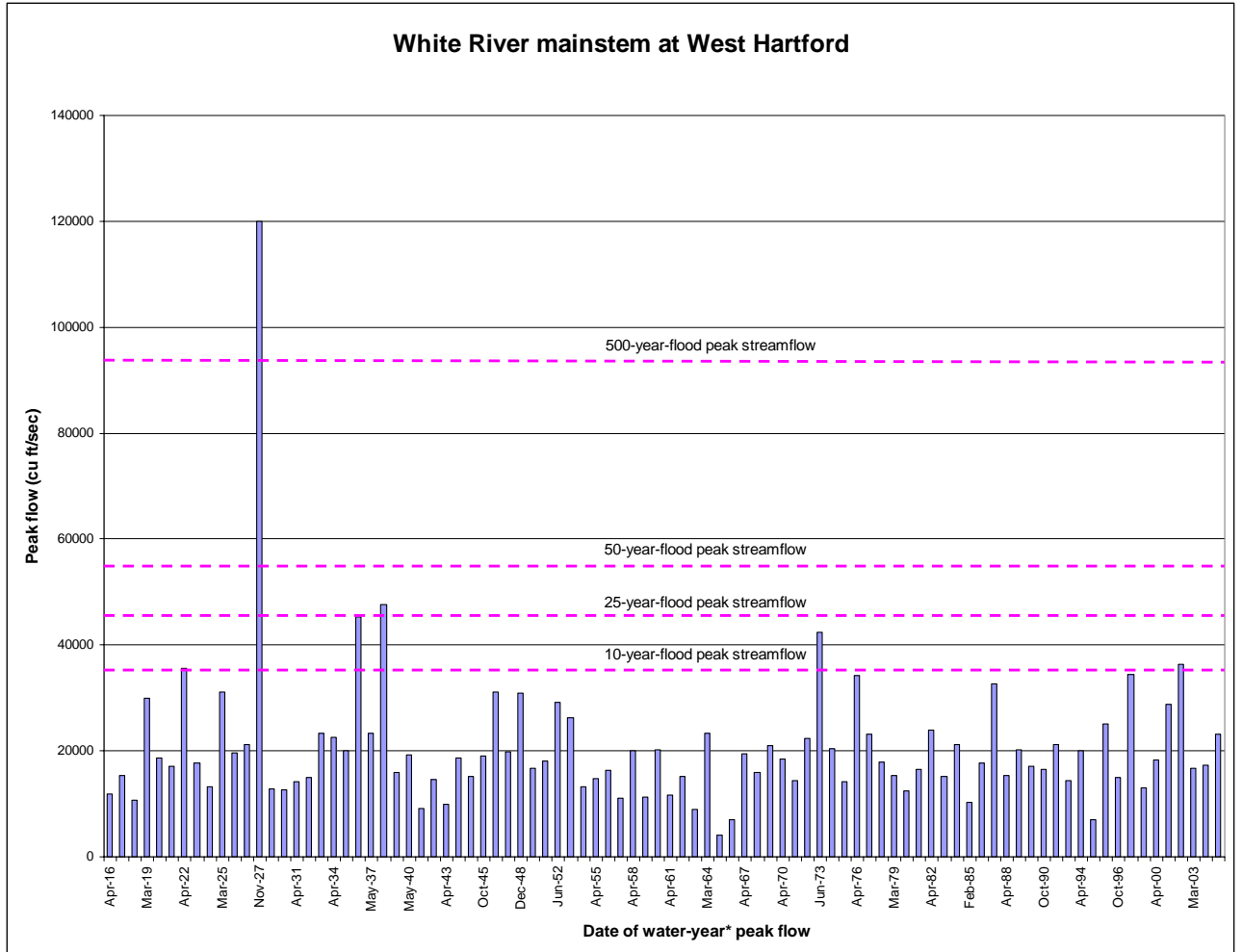
Figure 7. Annual and flood-level peak streamflows at the USGS continuous-record stream gage on the mainstem of the White River at West Hartford. (*Water years run from Oct. 1 to Sept. 30.)
