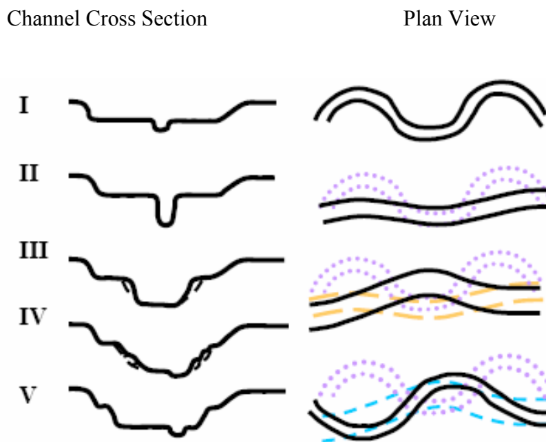
Figure 14. Channel evolution process showing channel downcutting or incision in Stage II (cross section), widening through Stages III and IV, and floodplain reestablishment in Stage V. Stages I and V represent equilibrium conditions. Plan view shows straightening and meander redevelopment that accompany cross-section changes, a flood-driven process taking place over decades (VT ANR 2007a).
