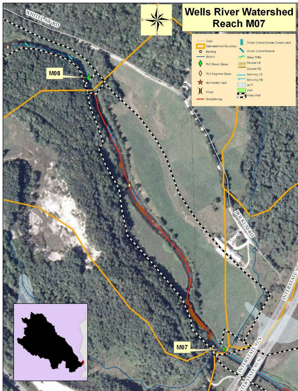
Figure 40: Wells River mainstem reach M07, Segments A and B
