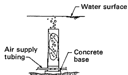
Helical aerator
