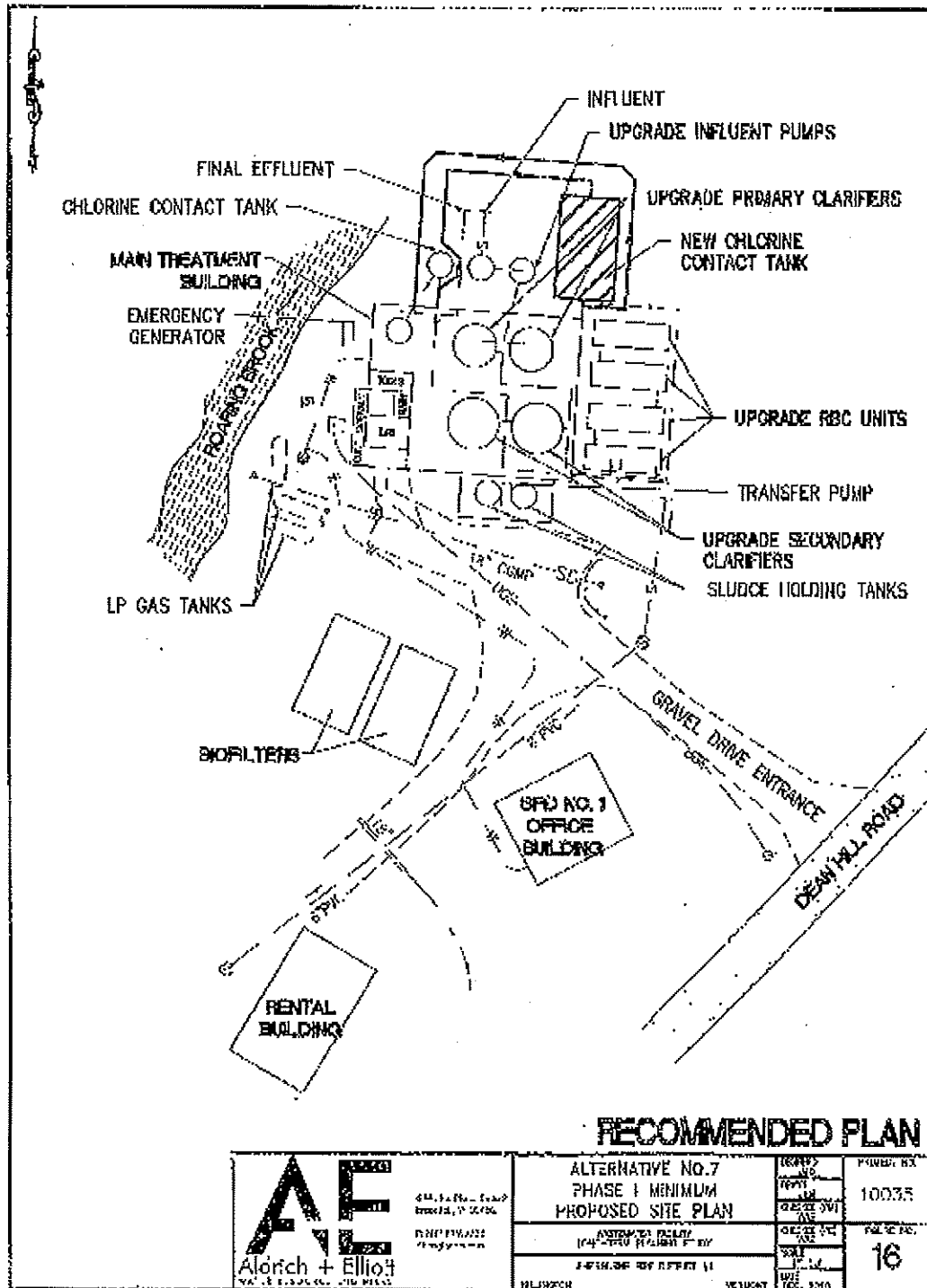
Figure 1, Proposed Project, Wastewater Facility Refurbishment, Phase 1, Sherburne Fire District No. 1
